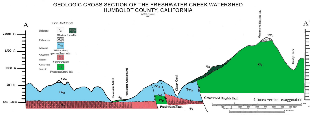
Figure 7. Geologic cross-section of the Freshwater watershed.
