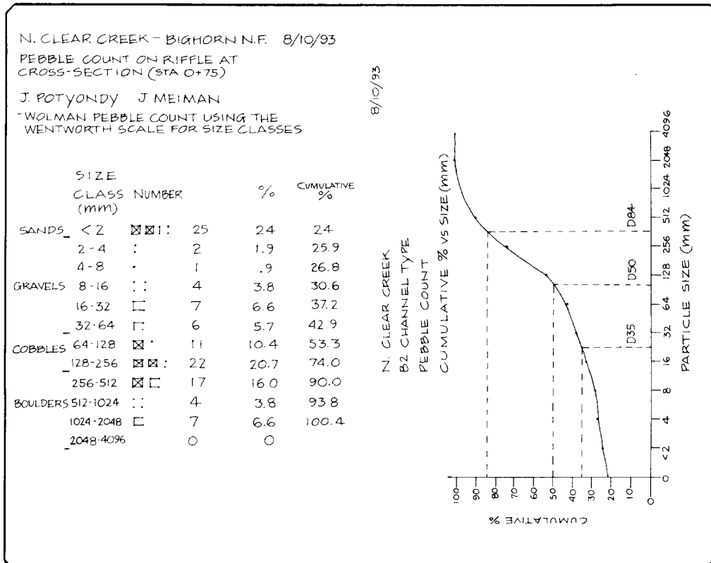
Figure 62. - Field plot of pebble count.
