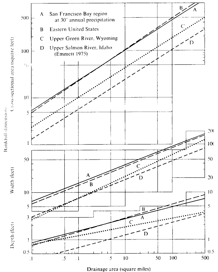
Figure 46. - Average values of bankfull channel dimensions as functions of drainage area for four regions. From: Water In Environmental Planning by Thomas Dunne and Luna B. Leopold. Copyright © 1978 by W.H. Freeman and Company. Reprinted with permission.
