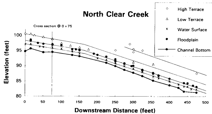
Figure 54. - Office plot of longitudinal profile survey.
